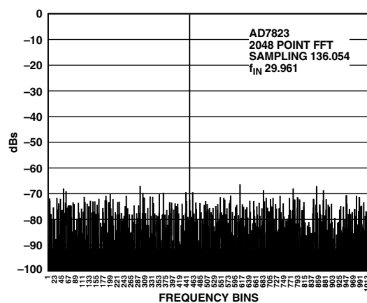
Figure 3. AD7823 SNR
